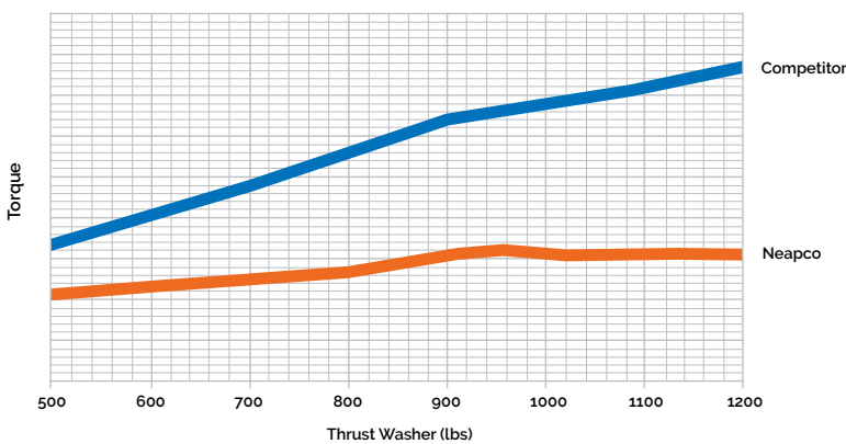
Articulation Torque Under Load
